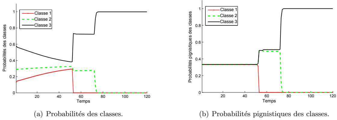
FIGURE 2.12: Classification Bayésienne vs classification crédale (application 1).
