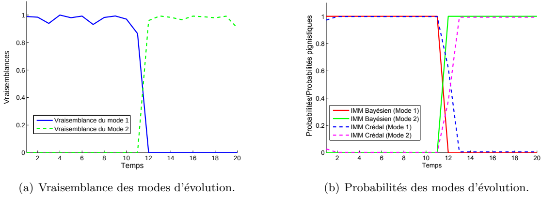
FIGURE 2.6: IMM classique vs IMM crédal [134].
