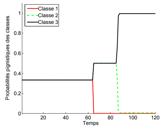
(b) Classification crédale locale.
